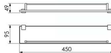
Porta Shampoo com Grade 29.QD01.CR
