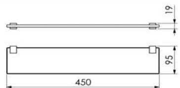
Porta Shampoo 29.QD00.CR
