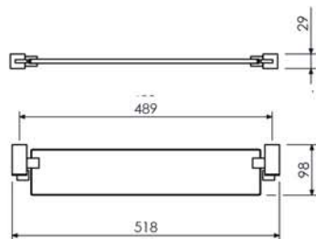
Porta Shampoo 29.SQ00.CR
