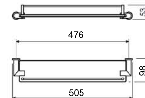
Porta Shampoo com Grade 29.PL01.CR
