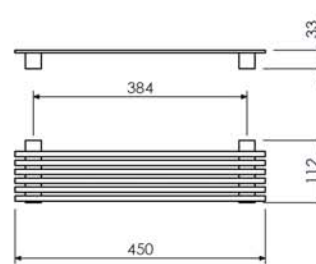
Porta Shampoo 29.TW00.CR
