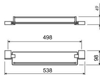
Porta Shampoo com Grade 29.UQ01.CR
