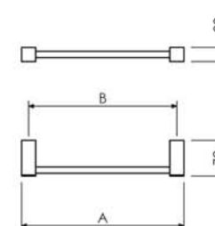
Toalheiro 20cm - A=229 B=200 07.KP01.CR 30cm - A=329 B=300 07.KP02.CR 45cm - A=479 B=450 07.KP03.CR 60cm - A=629 B=600 07.KP04.CR
