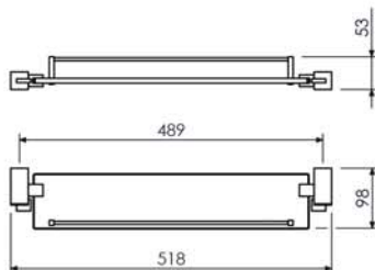
Porta Shampoo com Grade 29.SQ01.CR
