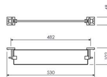
Porta Shampoo 29.TB00.CR
