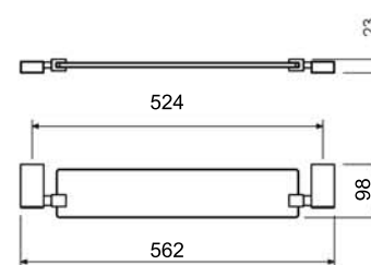
Porta Shampoo 29.OG00.CR
