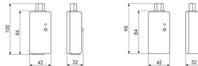
iOTT WiFi 2.4GHz 71.SO01.PF
